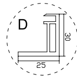
Frame cross-section
